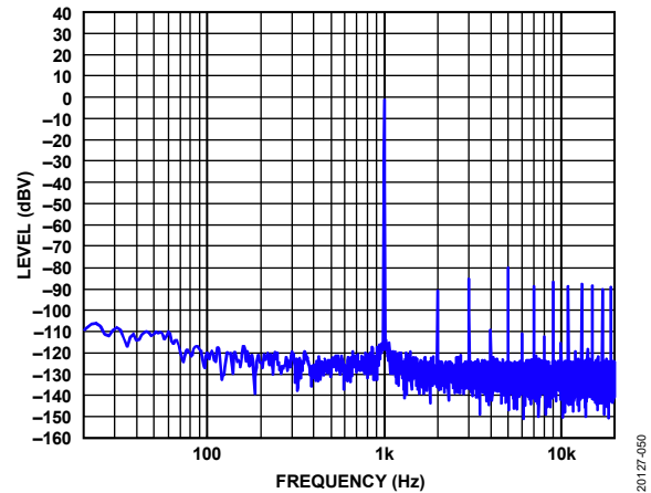
Figure 49. FFT, -1 dBV, Headphone Mode, Load = 16\ \Omega , f_s = 48\ \text{kHz} to 768\ \text{kHz} , Signal Path = AINx to HPOUTxx
